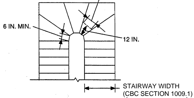
PLAN VIEW ALTERNATE USE OF WINDERS
