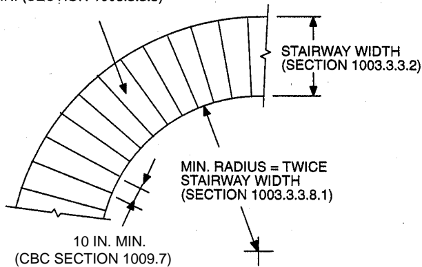
PLAN VIEW CIRCULAR STAIRWAY
